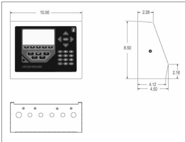
820i Universal Mount
