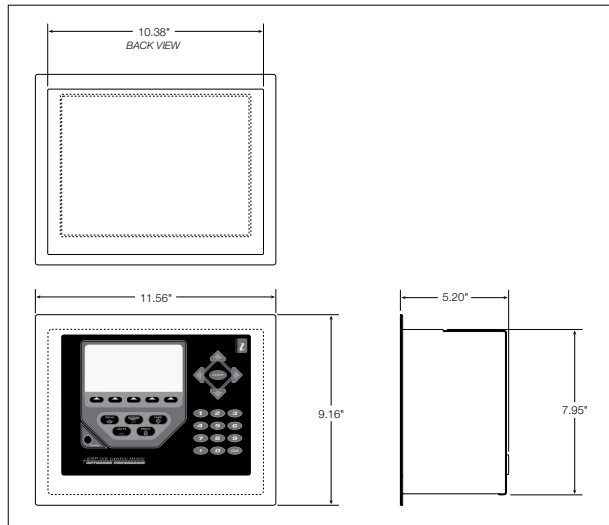
820i Panel Mount
